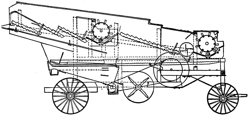
FIG. 6.—A bean thresher.
